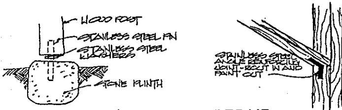
RESETTING FENCE POST
